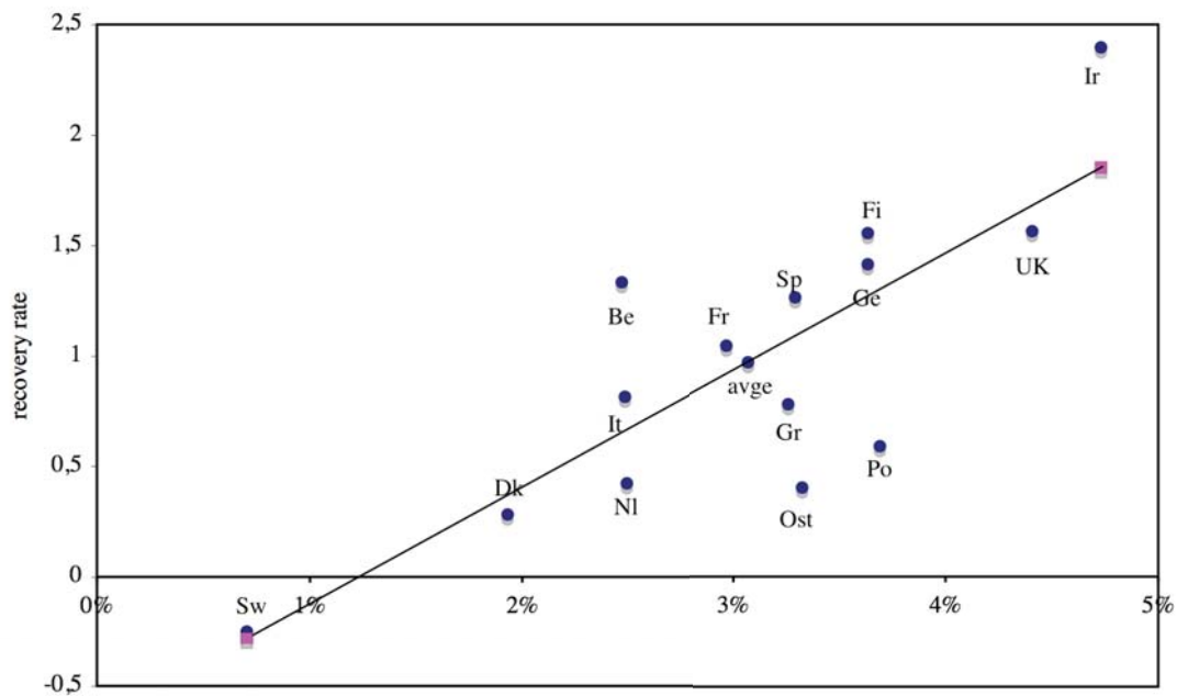
Figure 6: Recovery rate vs. \theta'
